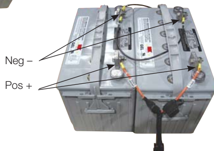
Figure 11 – Double Battery
