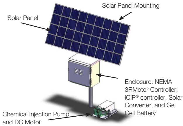
Figure 1 – iCIP® (Intelligent Chemical Injection Pump) Pump General Configuration
