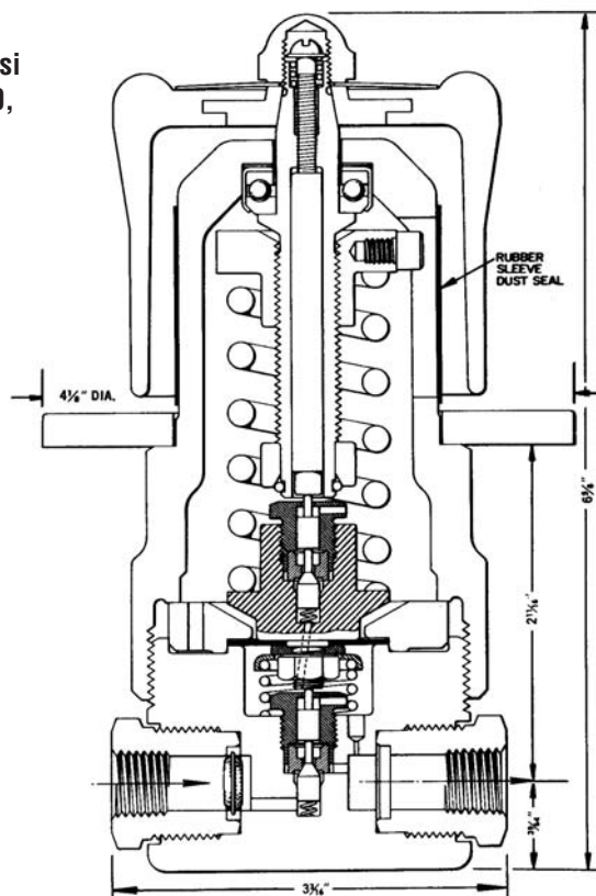
For mounting dimensions, see sheet W-15L-B01
