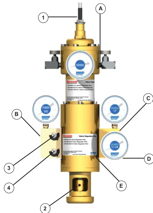
Figure 4.0 - Becker Model VRP-600-B-CH pressure control system. The VRP-B-CH is specifically designed for use in natural gas pressure regulation and provides a simple, economical alternative to the controller/positioner combination.
