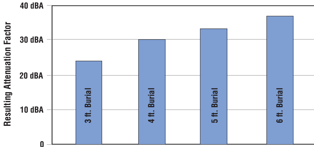
Figure 5 - Noise Attenuation as Factor of Depth.
